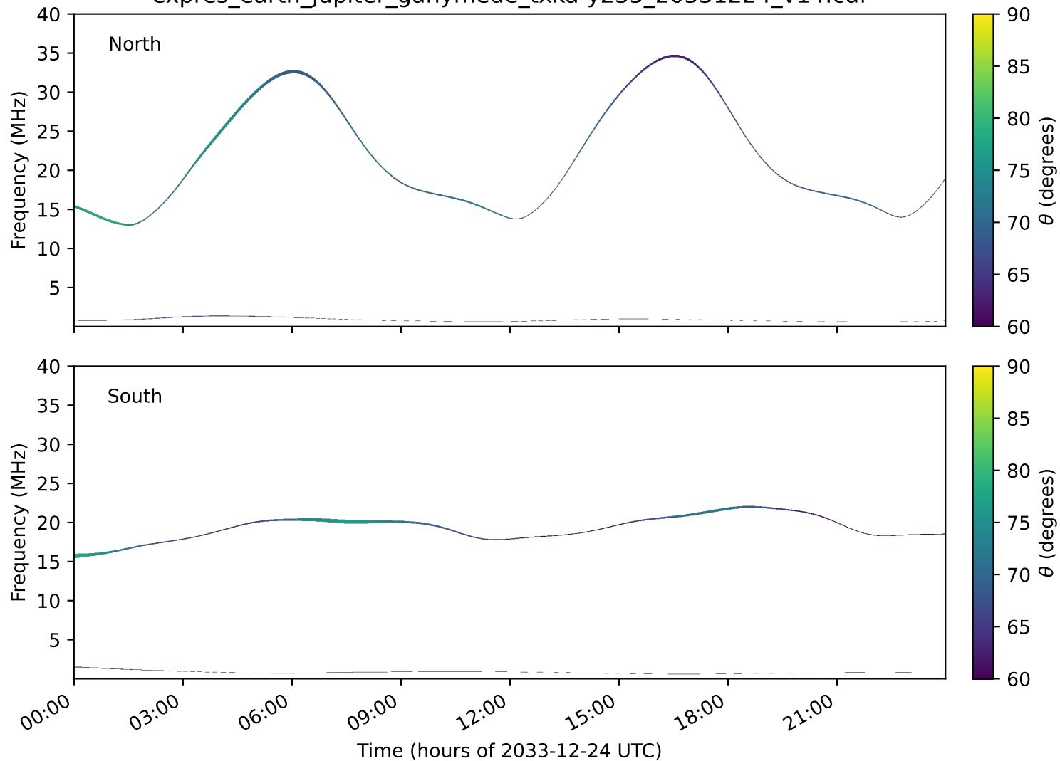
expres_earth_jupiter_ganymede_txka-y235_20331224_v14.cdf
