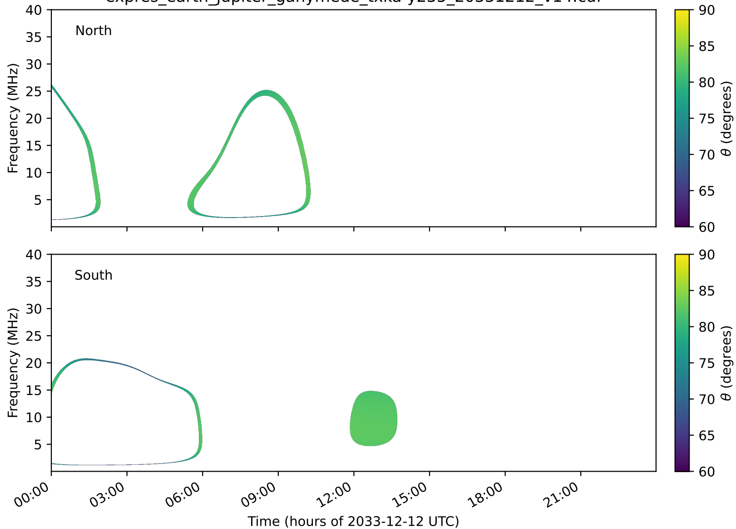
expres_earth_jupiter_ganymede_txka-y235_20331212_v14.cdf
