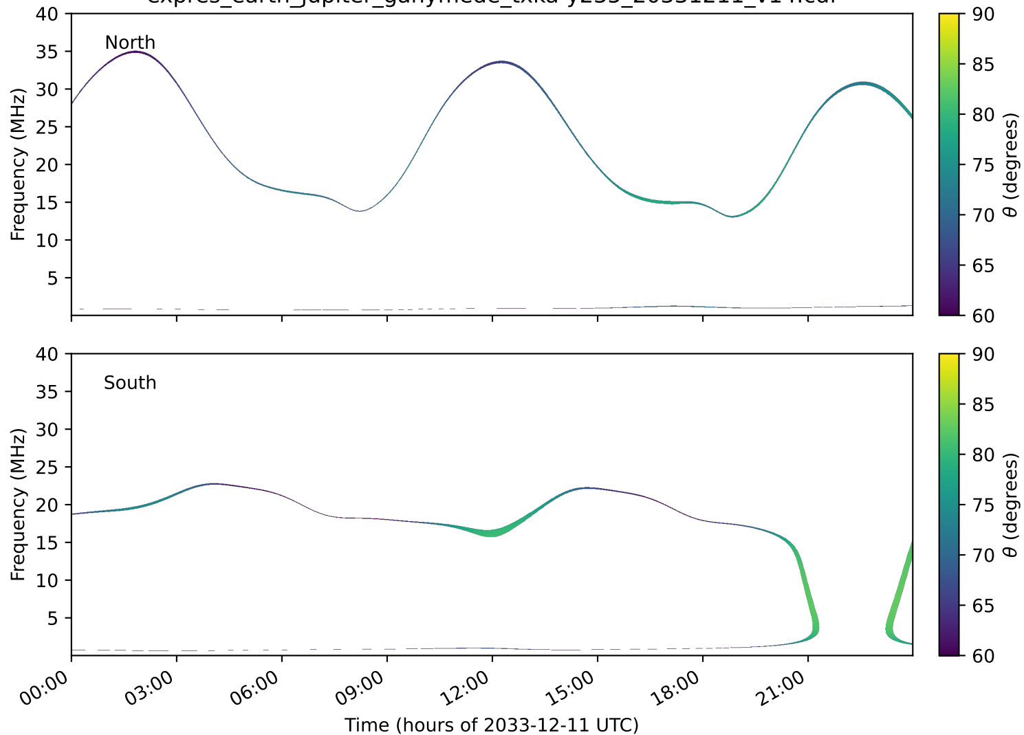
expres_earth_jupiter_ganymede_txka-y235_20331211_v14.cdf
