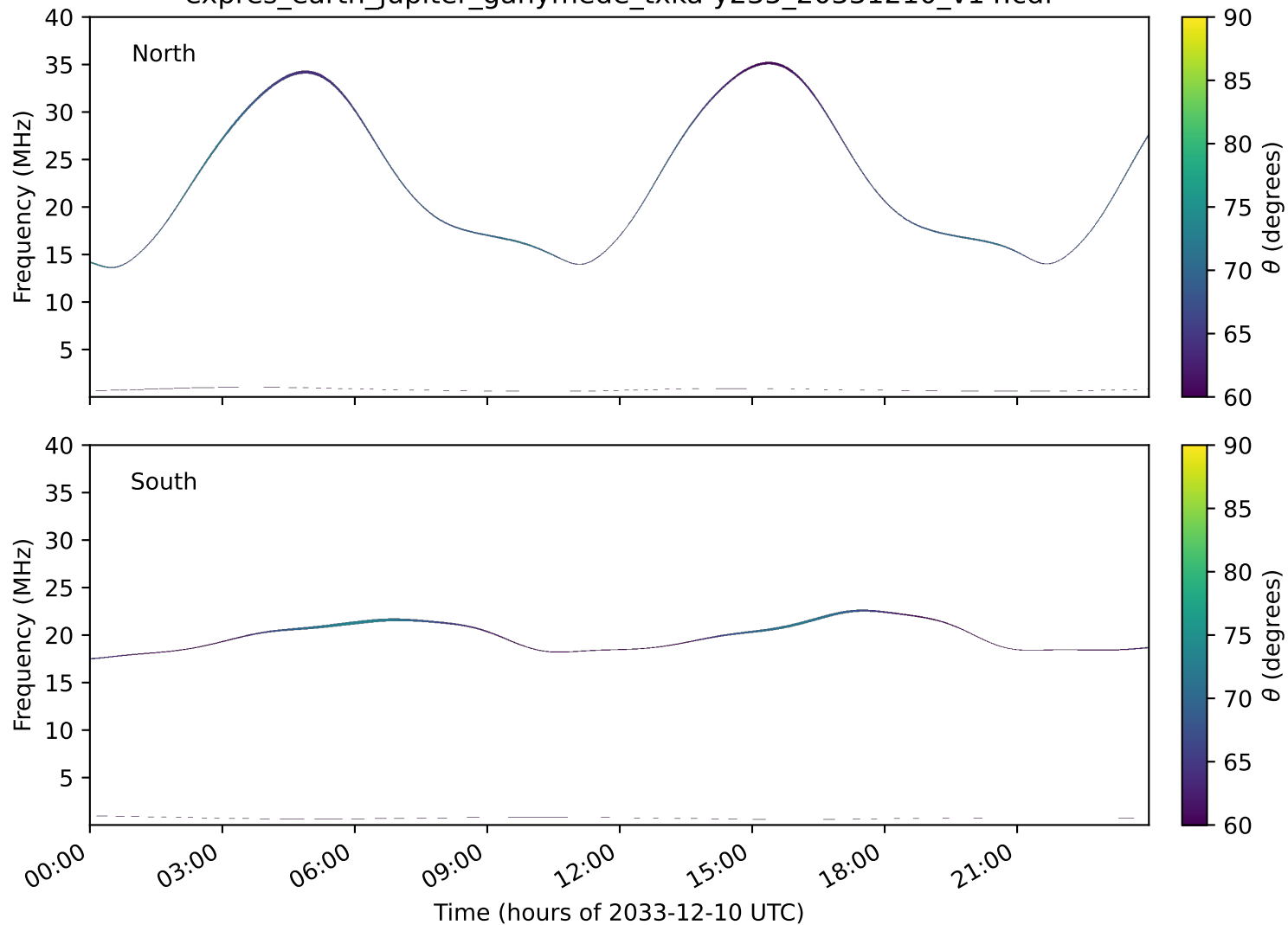
expres_earth_jupiter_ganymede_txka-y235_20331210_v14.cdf
