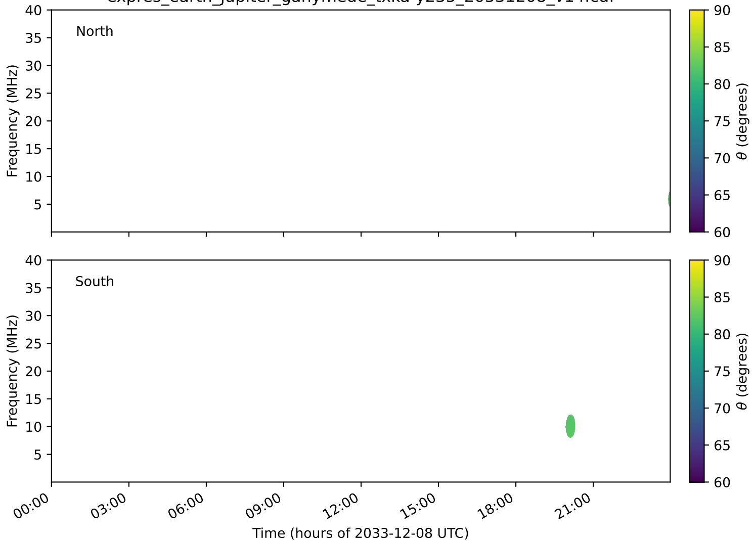
expres_earth_jupiter_ganymede_txka-y235_20331208_v14.cdf
