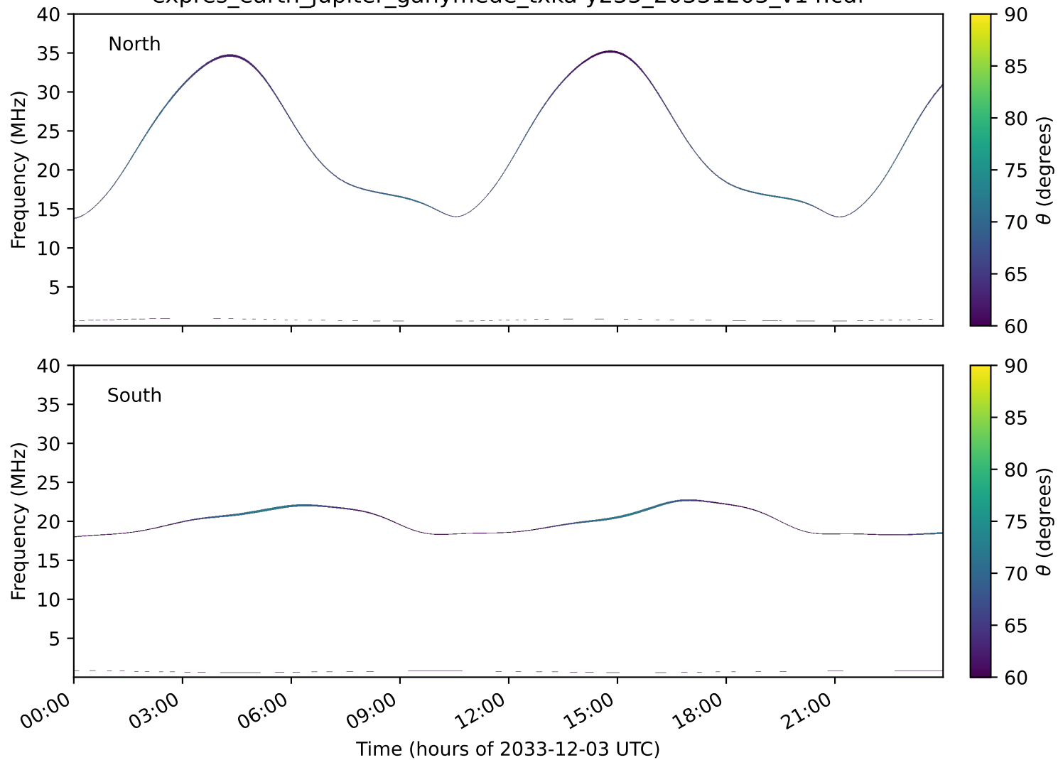
expres_earth_jupiter_ganymede_txka-y235_20331203_v14.cdf
