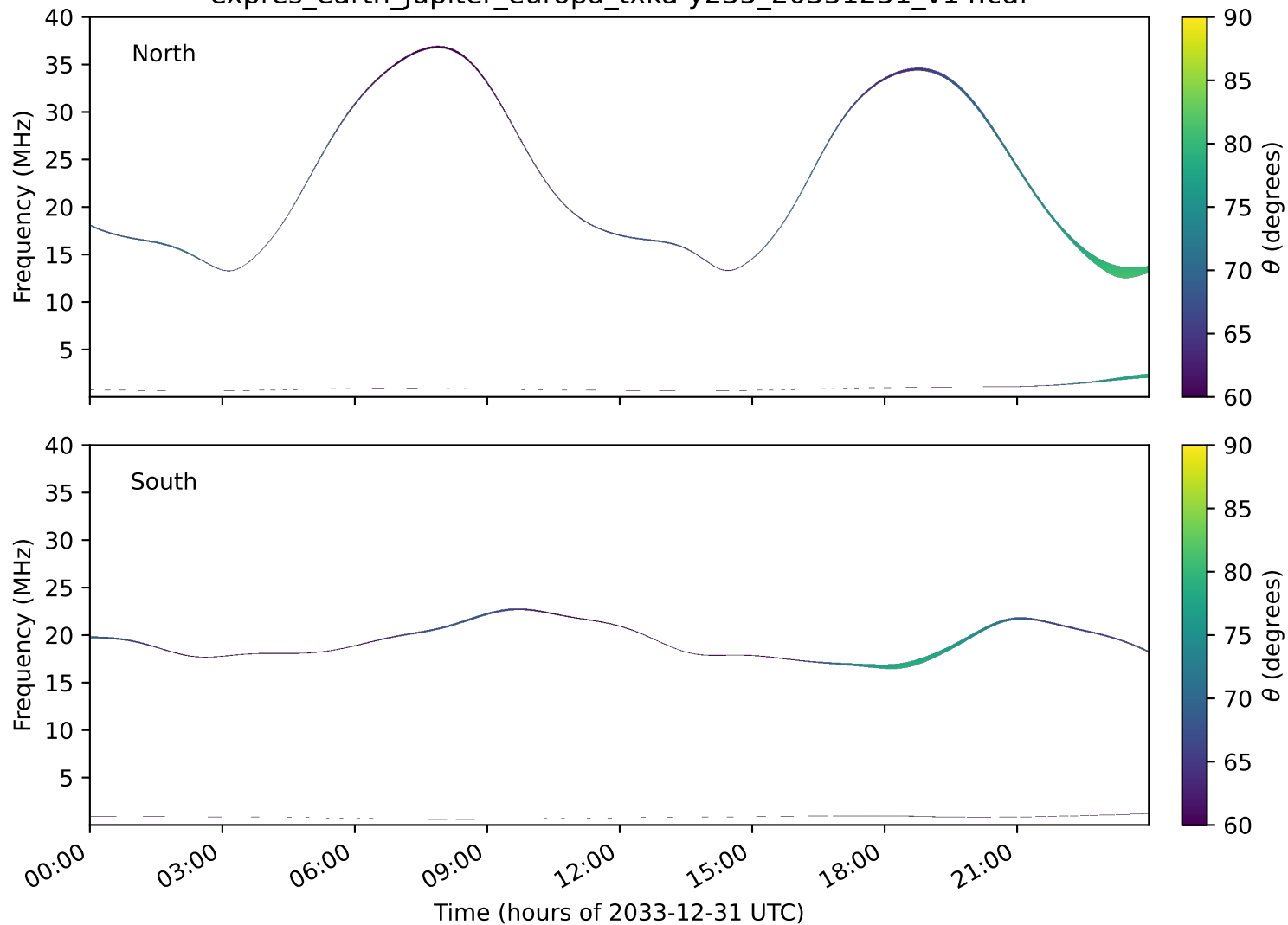
expres_earth_jupiter_europa_txka-y235_20331231_v14.cdf
