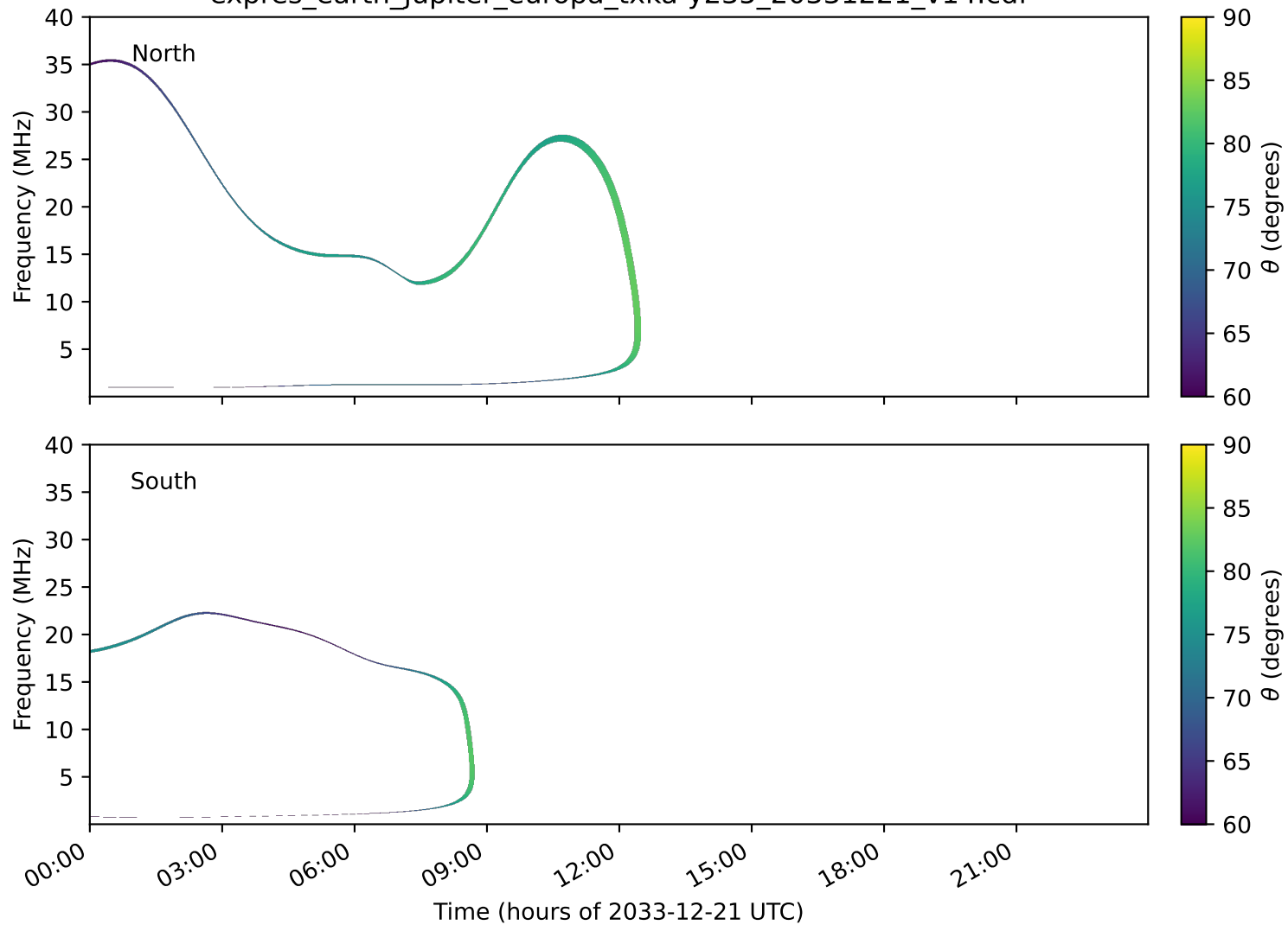
expres_earth_jupiter_europa_txka-y235_20331221_v14.cdf
