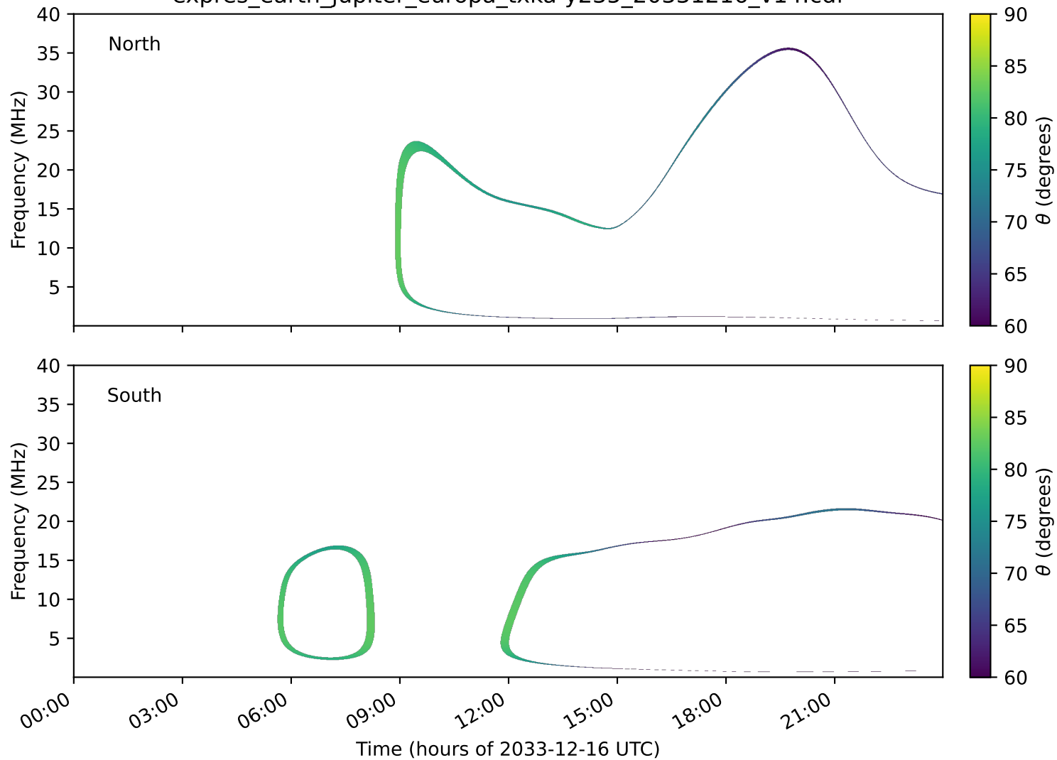
expres_earth_jupiter_europa_txka-y235_20331216_v14.cdf
