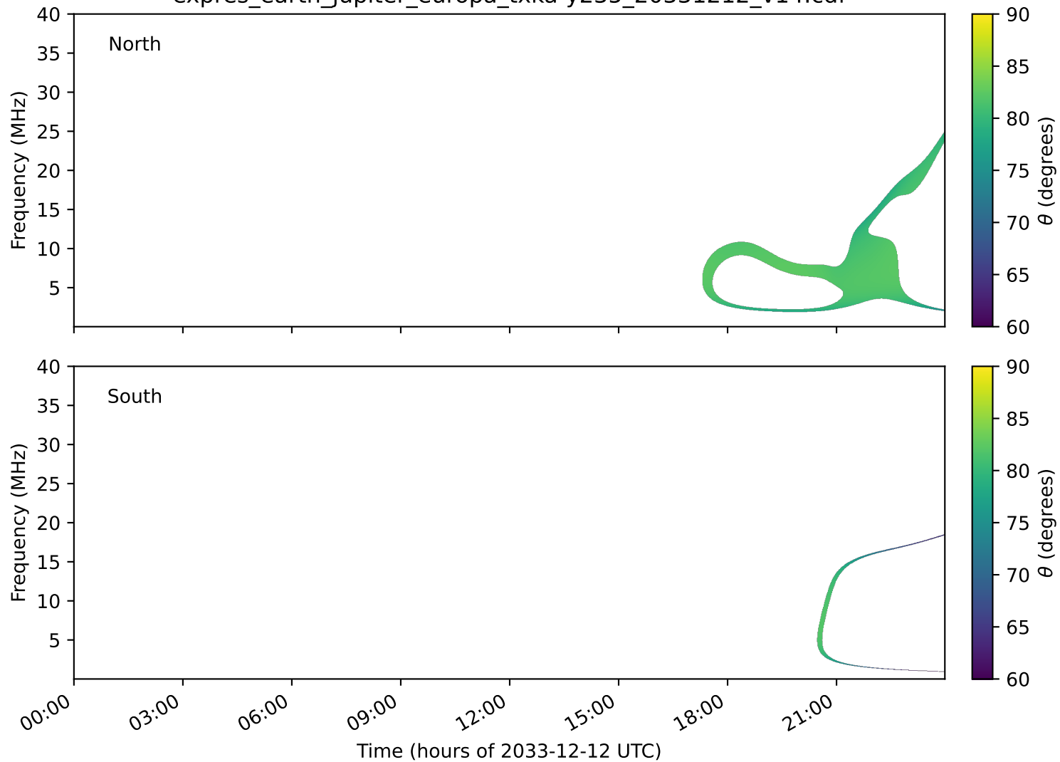
expres_earth_jupiter_europa_txka-y235_20331212_v14.cdf
