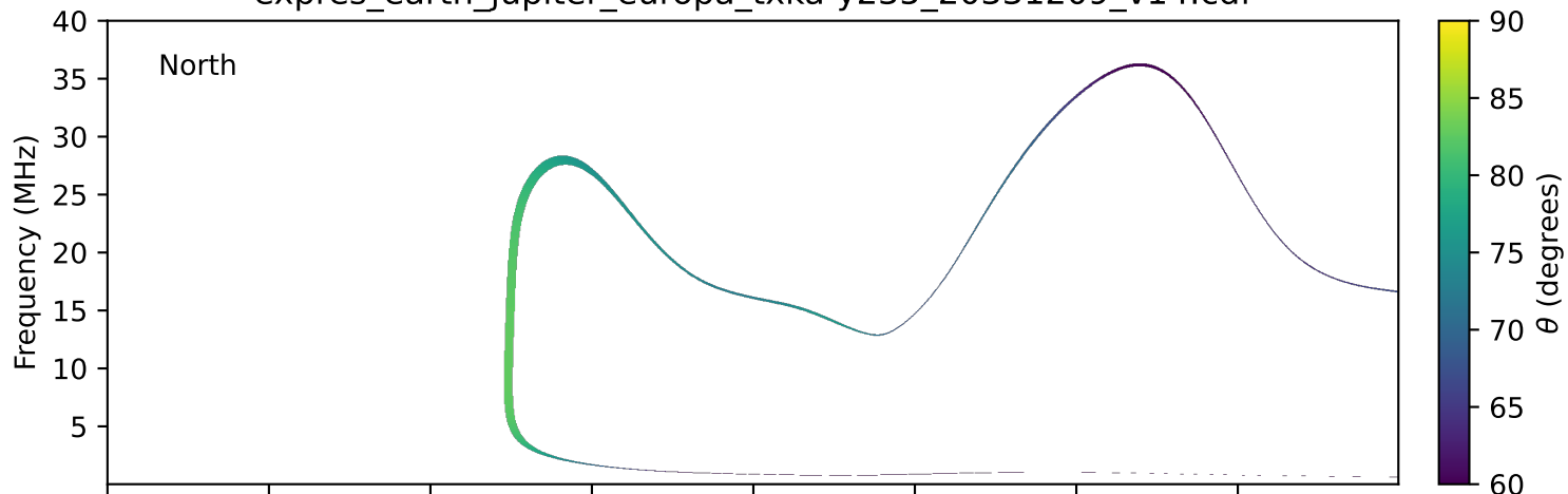
expres_earth_jupiter_europa_txka-y235_20331209_v14.cdf
