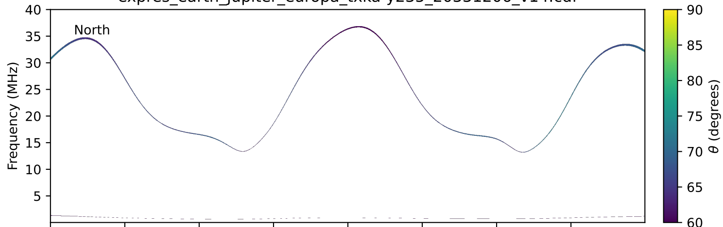
expres_earth_jupiter_europa_txka-y235_20331206_v14.cdf
