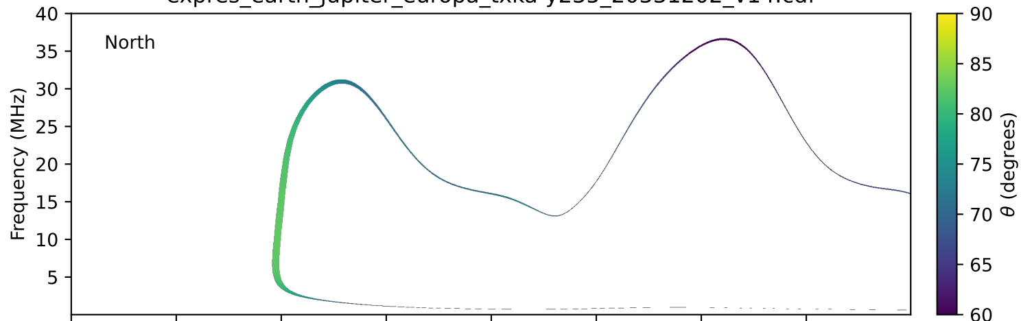
expres_earth_jupiter_europa_txka-y235_20331202_v14.cdf
