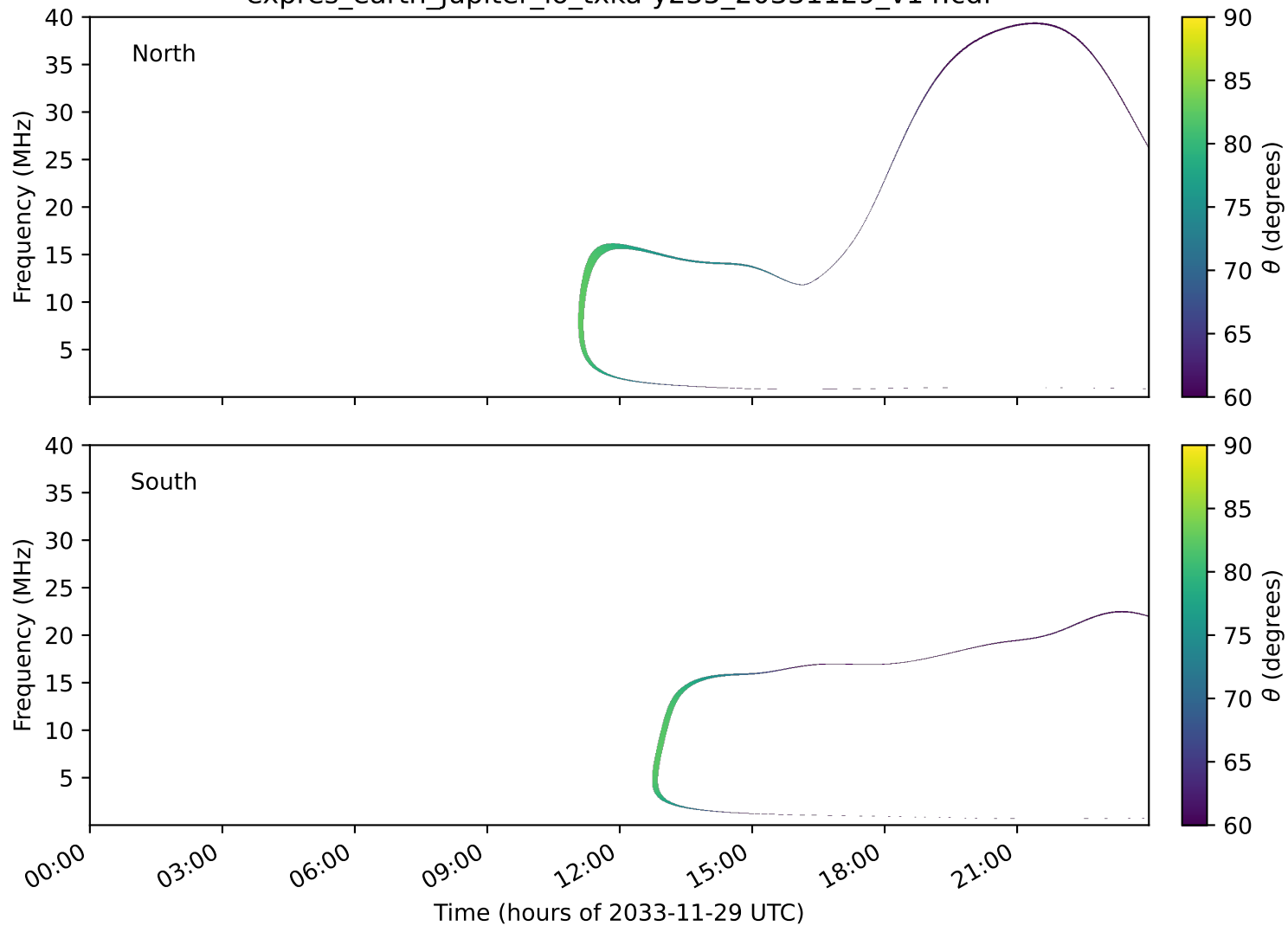
expres_earth_jupiter_io_txka-y235_20331129_v14.cdf
