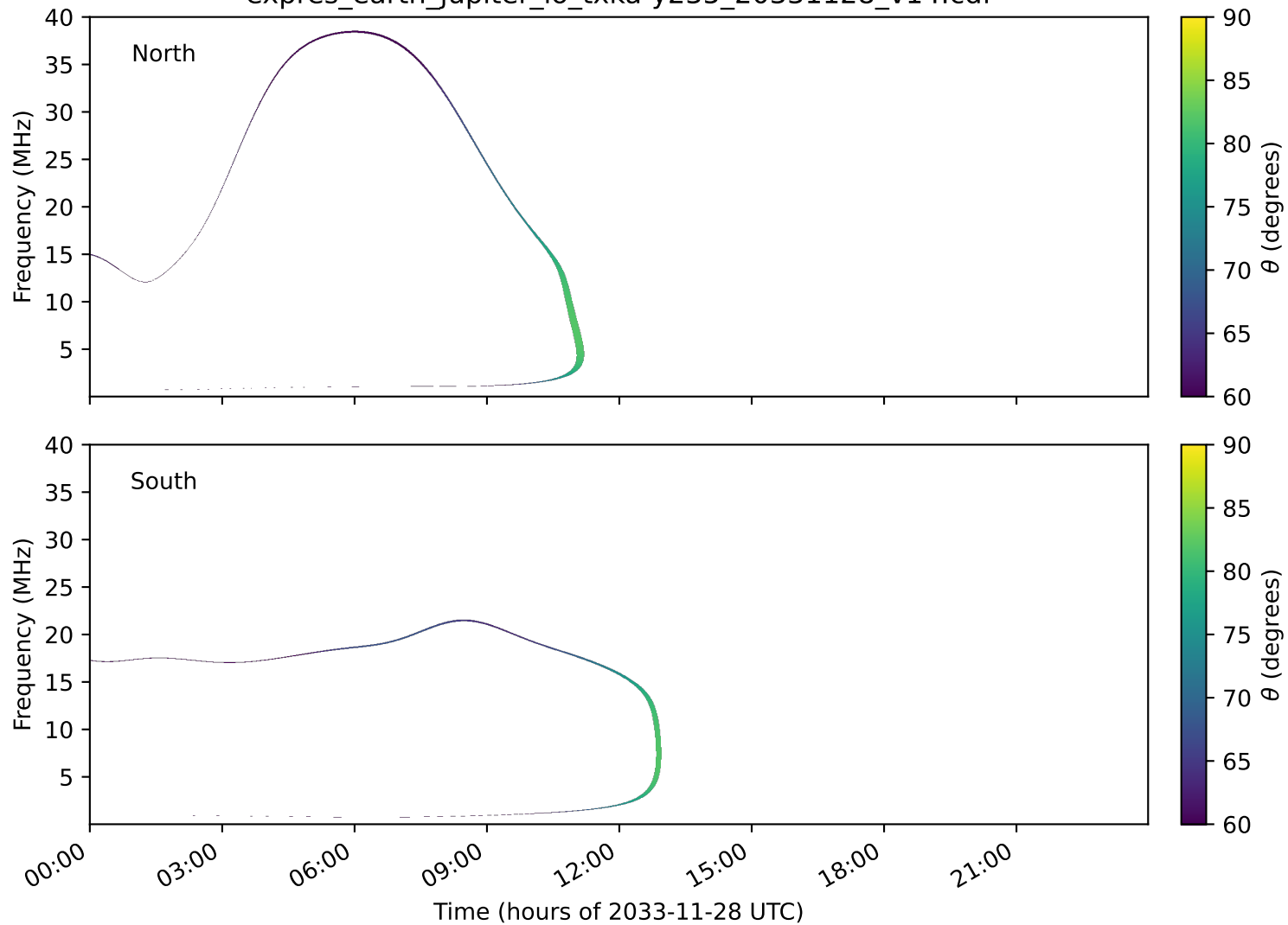
expres_earth_jupiter_io_txka-y235_20331128_v14.cdf
