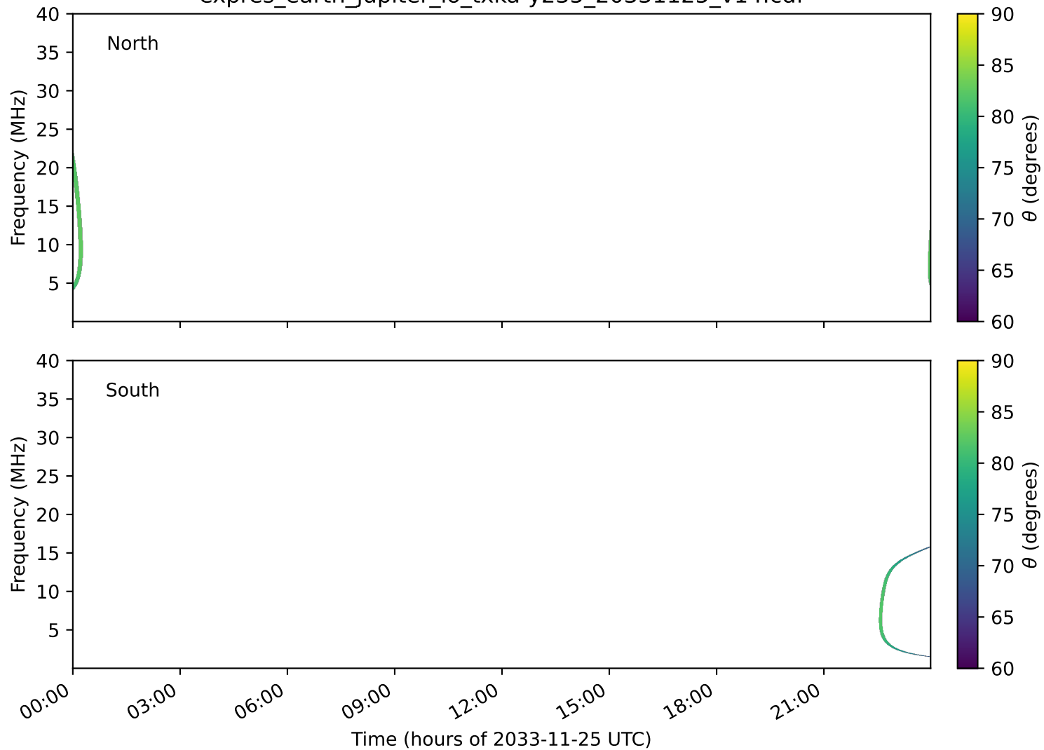
expres_earth_jupiter_io_txka-y235_20331125_v14.cdf
