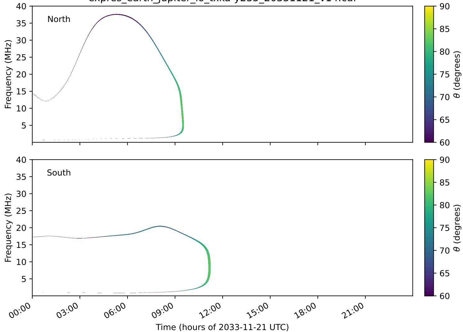
expres_earth_jupiter_io_txka-y235_20331121_v14.cdf
