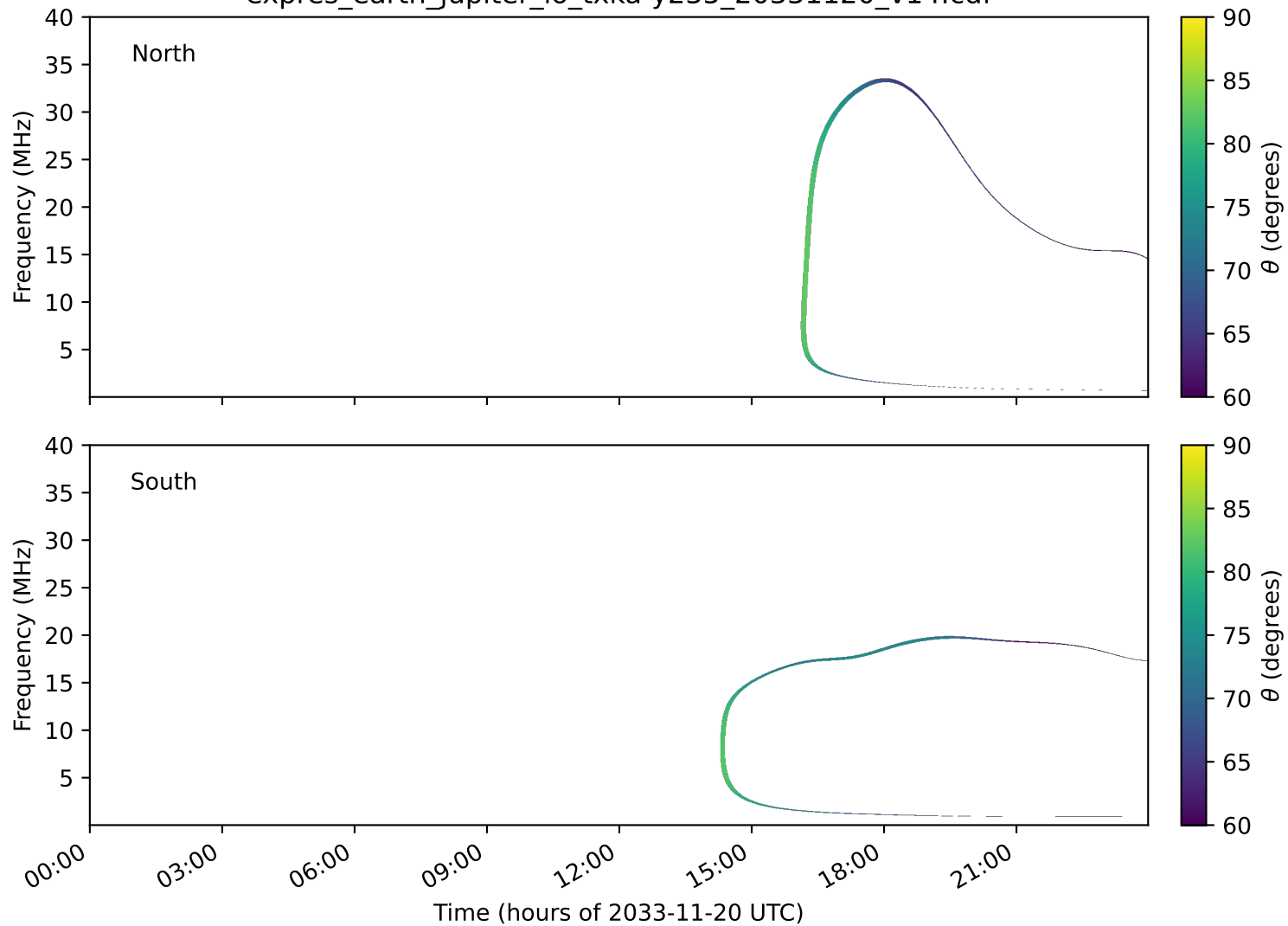
expres_earth_jupiter_io_txka-y235_20331120_v14.cdf
