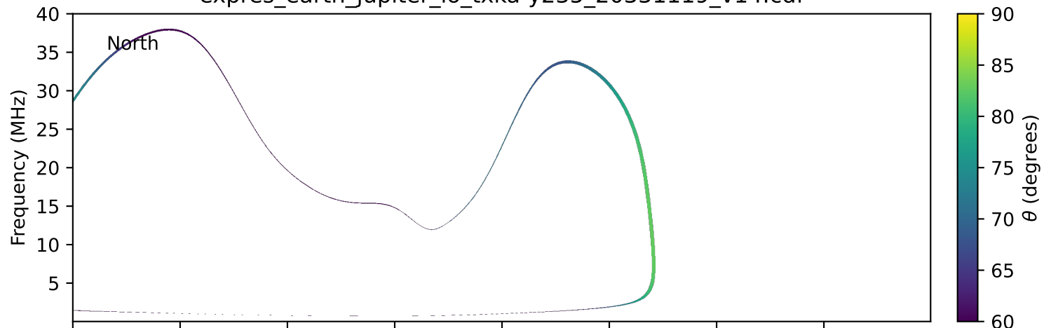
expres_earth_jupiter_io_txka-y235_20331119_v14.cdf
