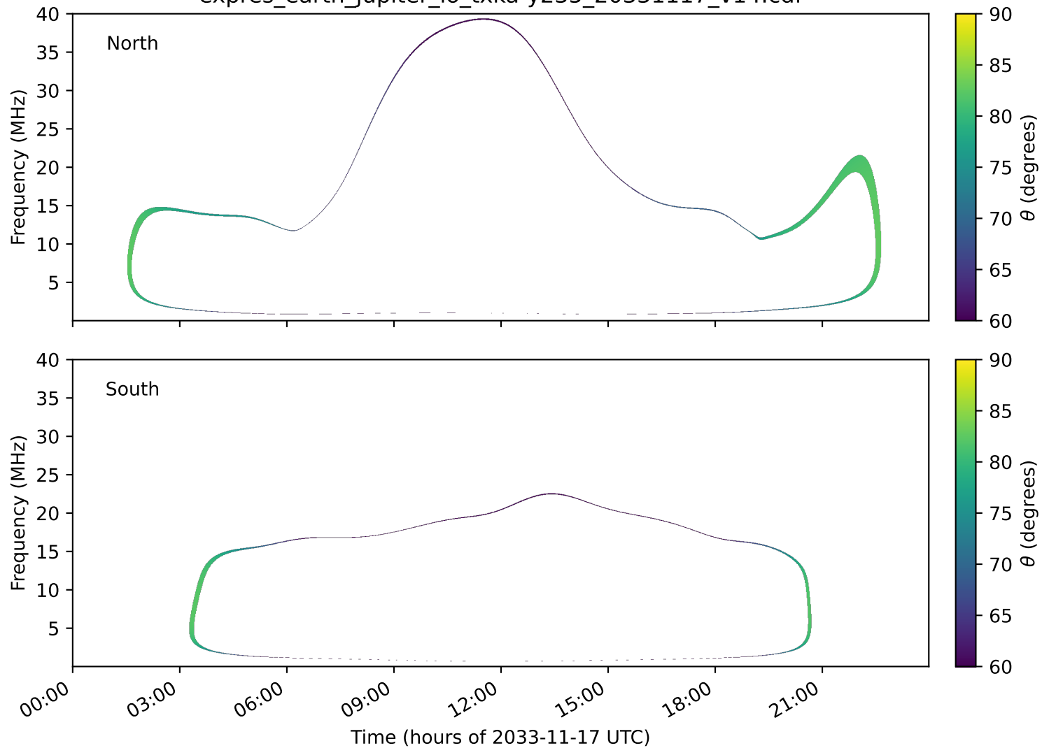
expres_earth_jupiter_io_txka-y235_20331117_v14.cdf
