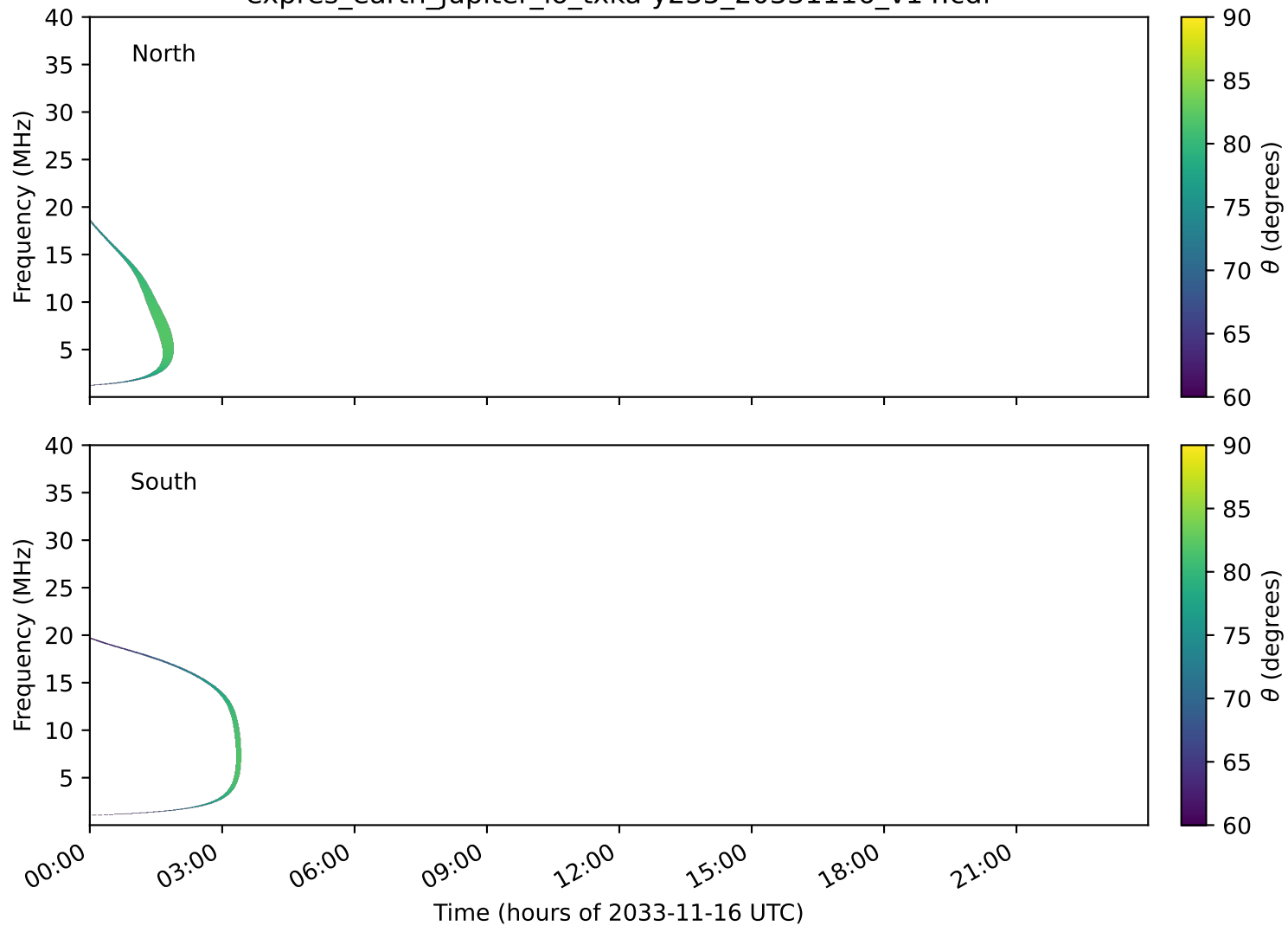
expres_earth_jupiter_io_txka-y235_20331116_v14.cdf
