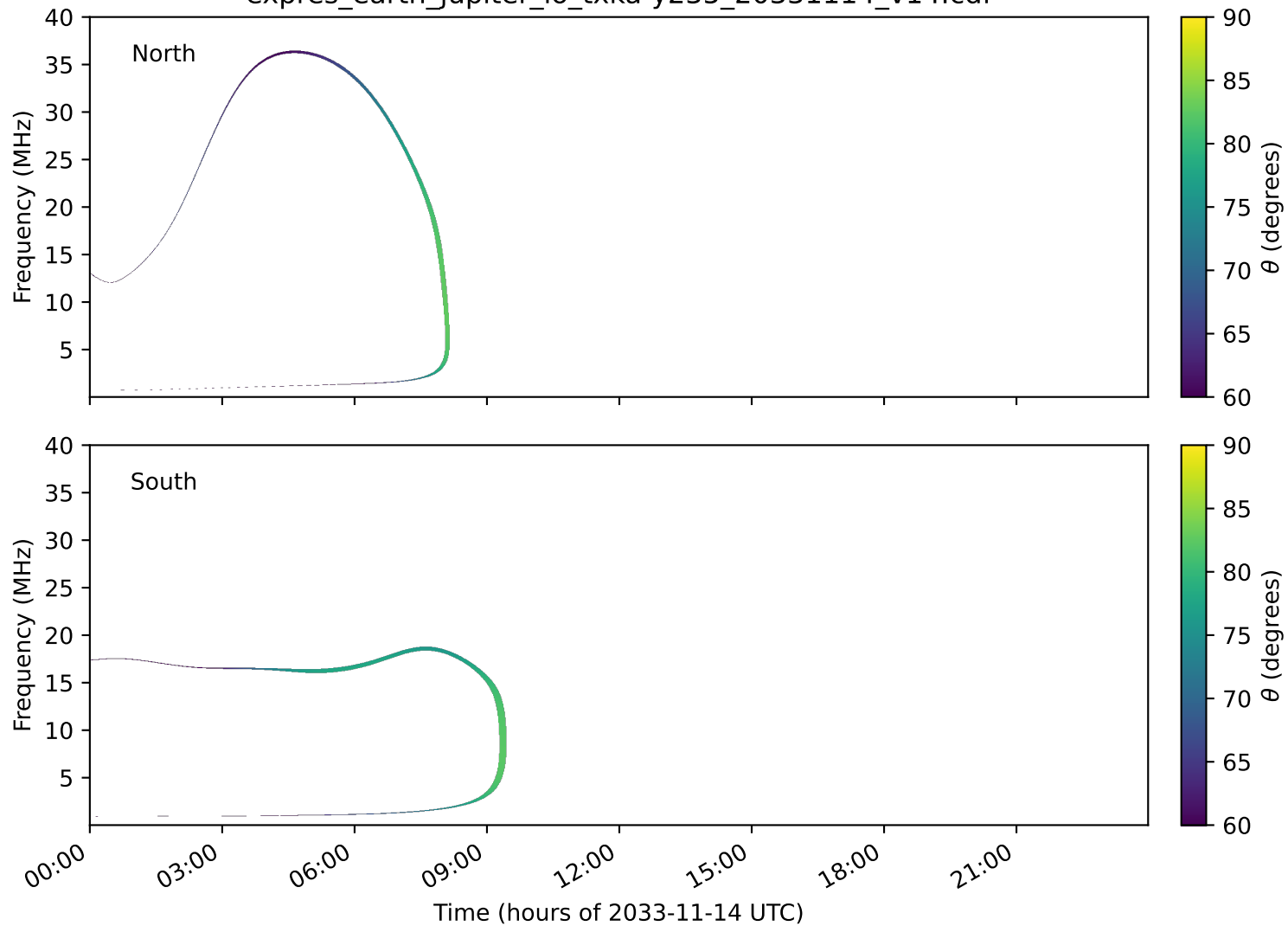
expres_earth_jupiter_io_txka-y235_20331114_v14.cdf
