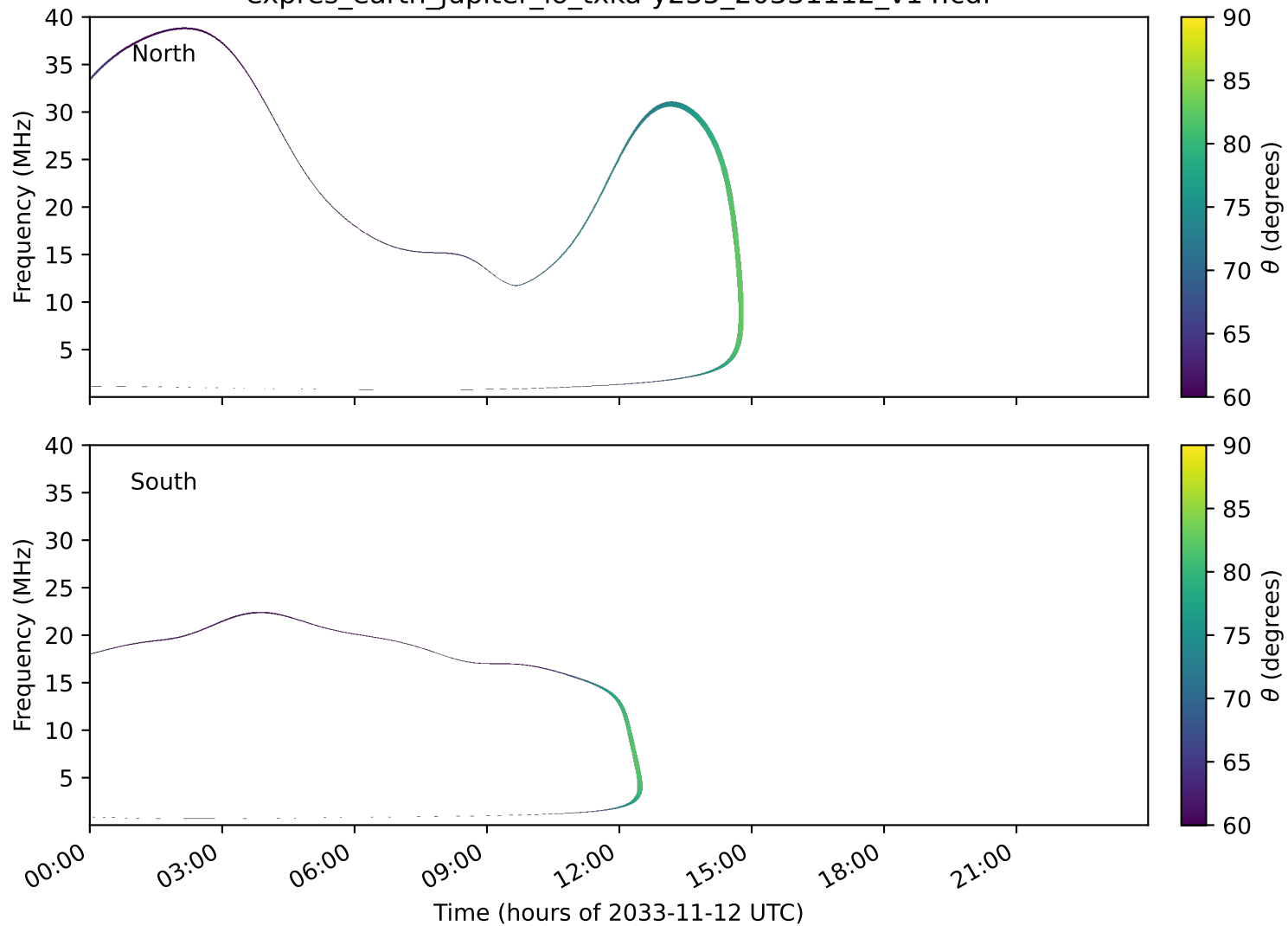
expres_earth_jupiter_io_txka-y235_20331112_v14.cdf
