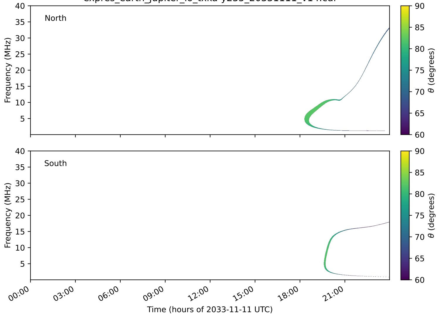
expres_earth_jupiter_io_txka-y235_20331111_v14.cdf
