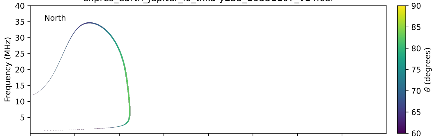
expres_earth_jupiter_io_txka-y235_20331107_v14.cdf
