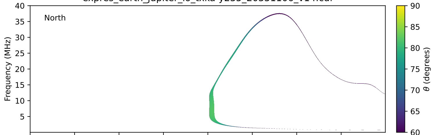
expres_earth_jupiter_io_txka-y235_20331106_v14.cdf
