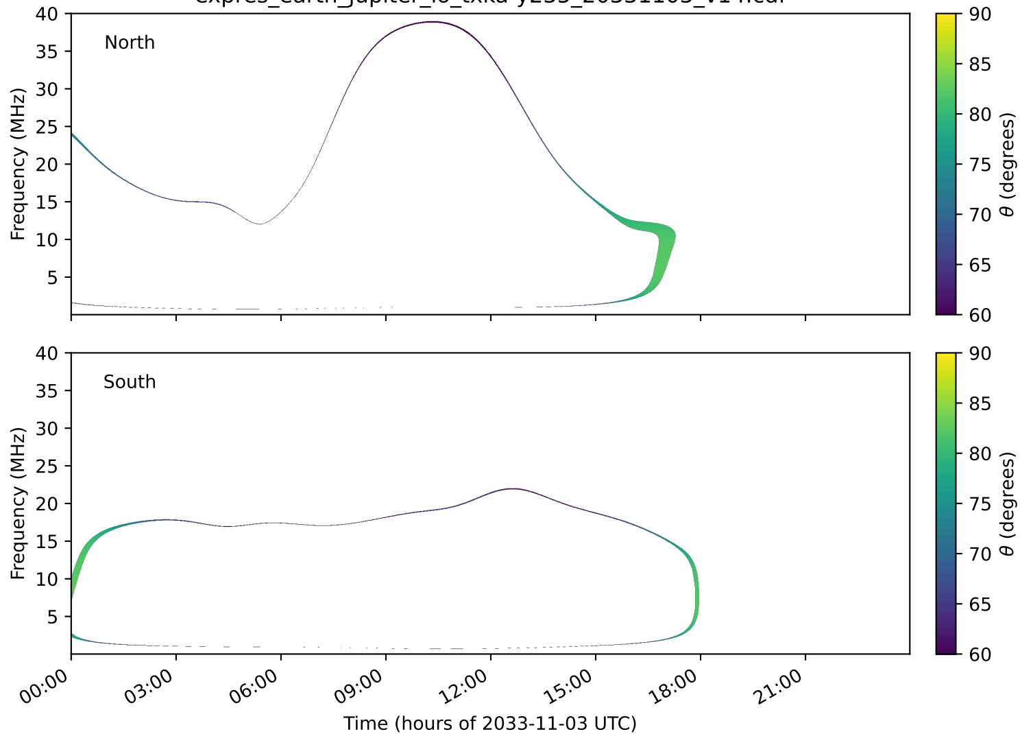
expres_earth_jupiter_io_txka-y235_20331103_v14.cdf
