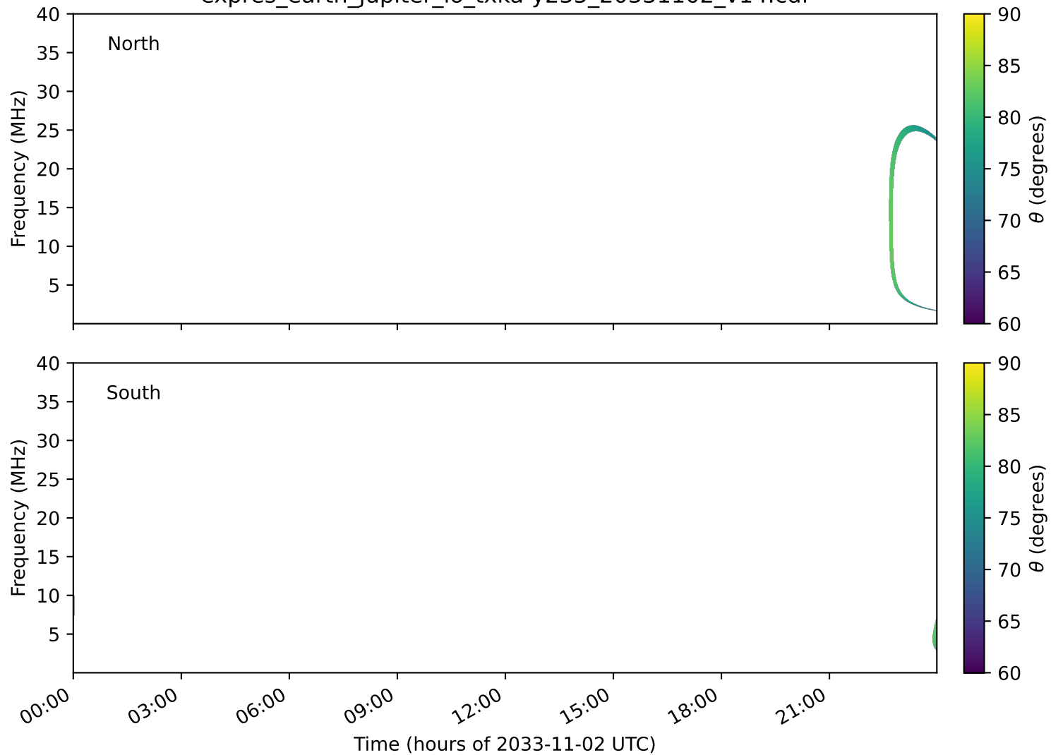
expres_earth_jupiter_io_txka-y235_20331102_v14.cdf
