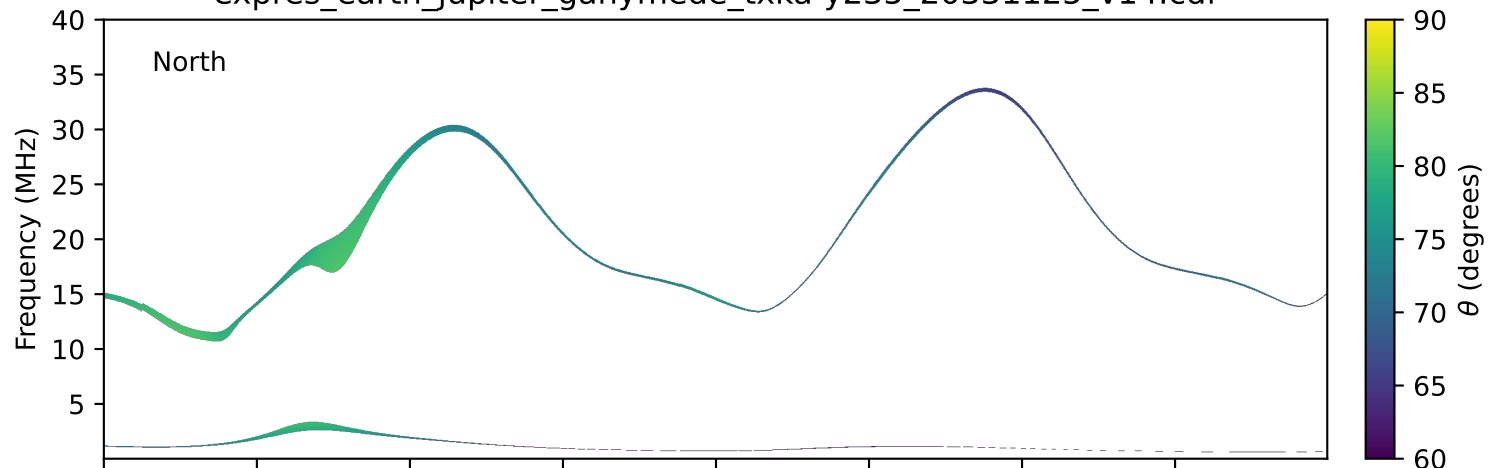
expres_earth_jupiter_ganymede_txka-y235_20331125_v14.cdf
