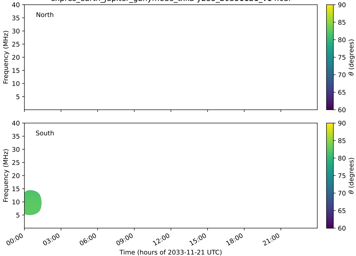
expres_earth_jupiter_ganymede_txka-y235_20331121_v14.cdf
