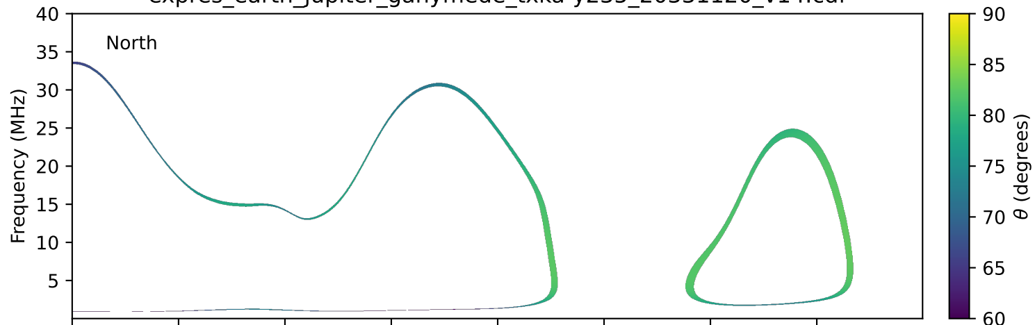
expres_earth_jupiter_ganymede_txka-y235_20331120_v14.cdf
