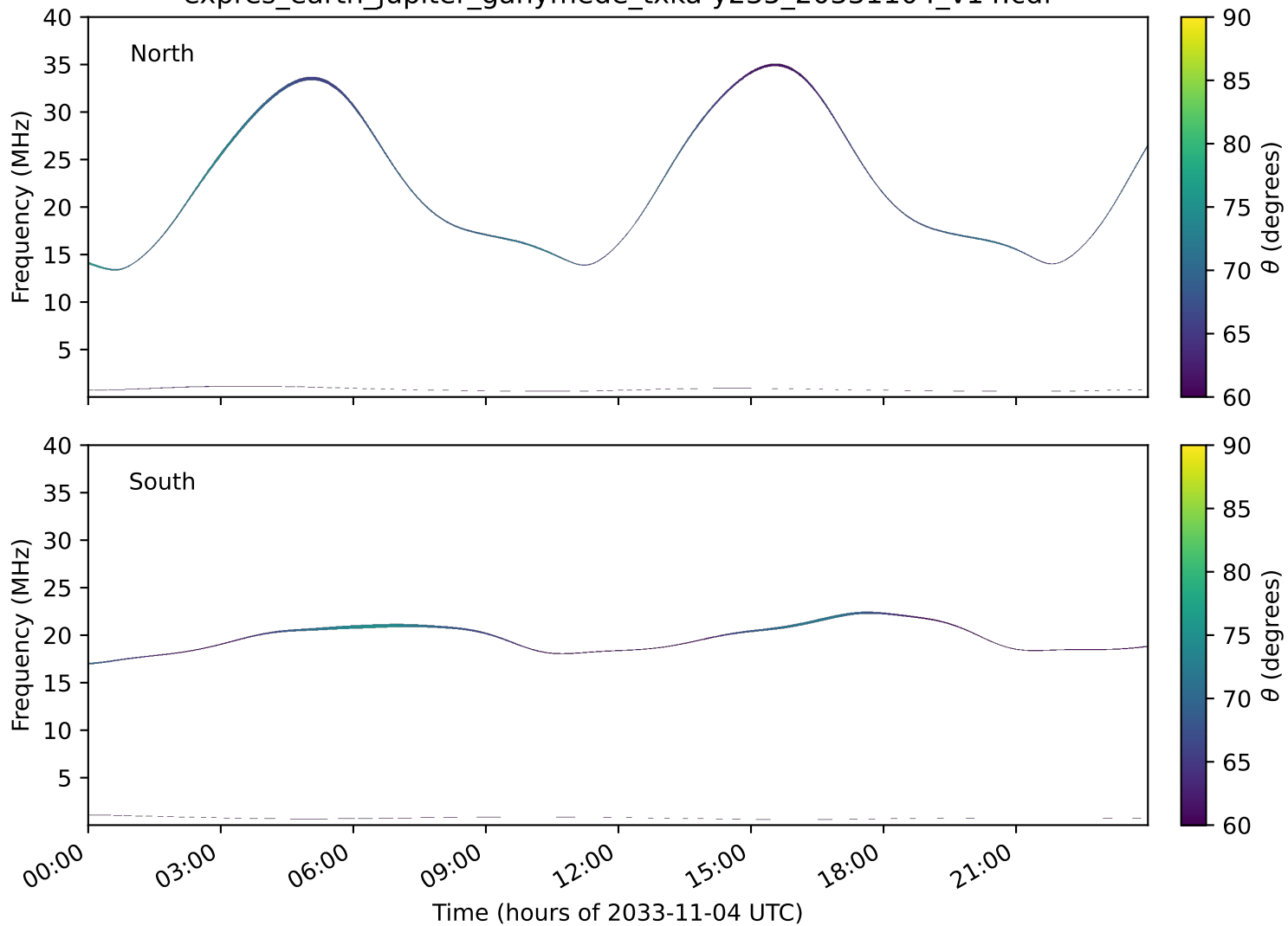
expres_earth_jupiter_ganymede_txka-y235_20331104_v14.cdf
