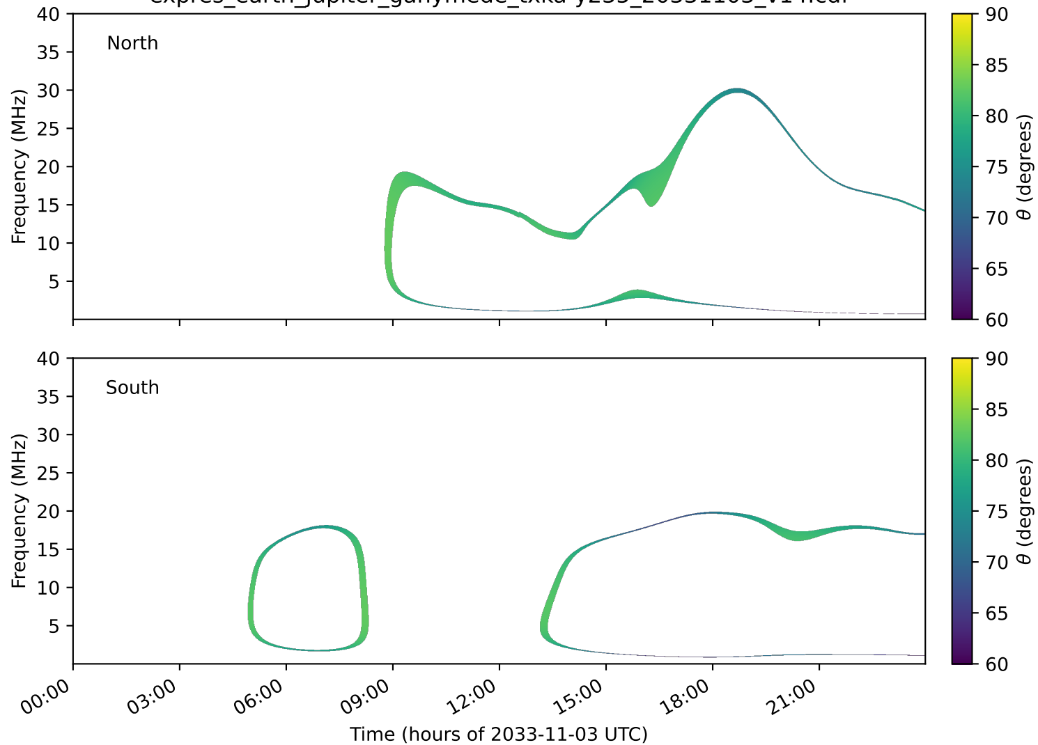
expres_earth_jupiter_ganymede_txka-y235_20331103_v14.cdf
