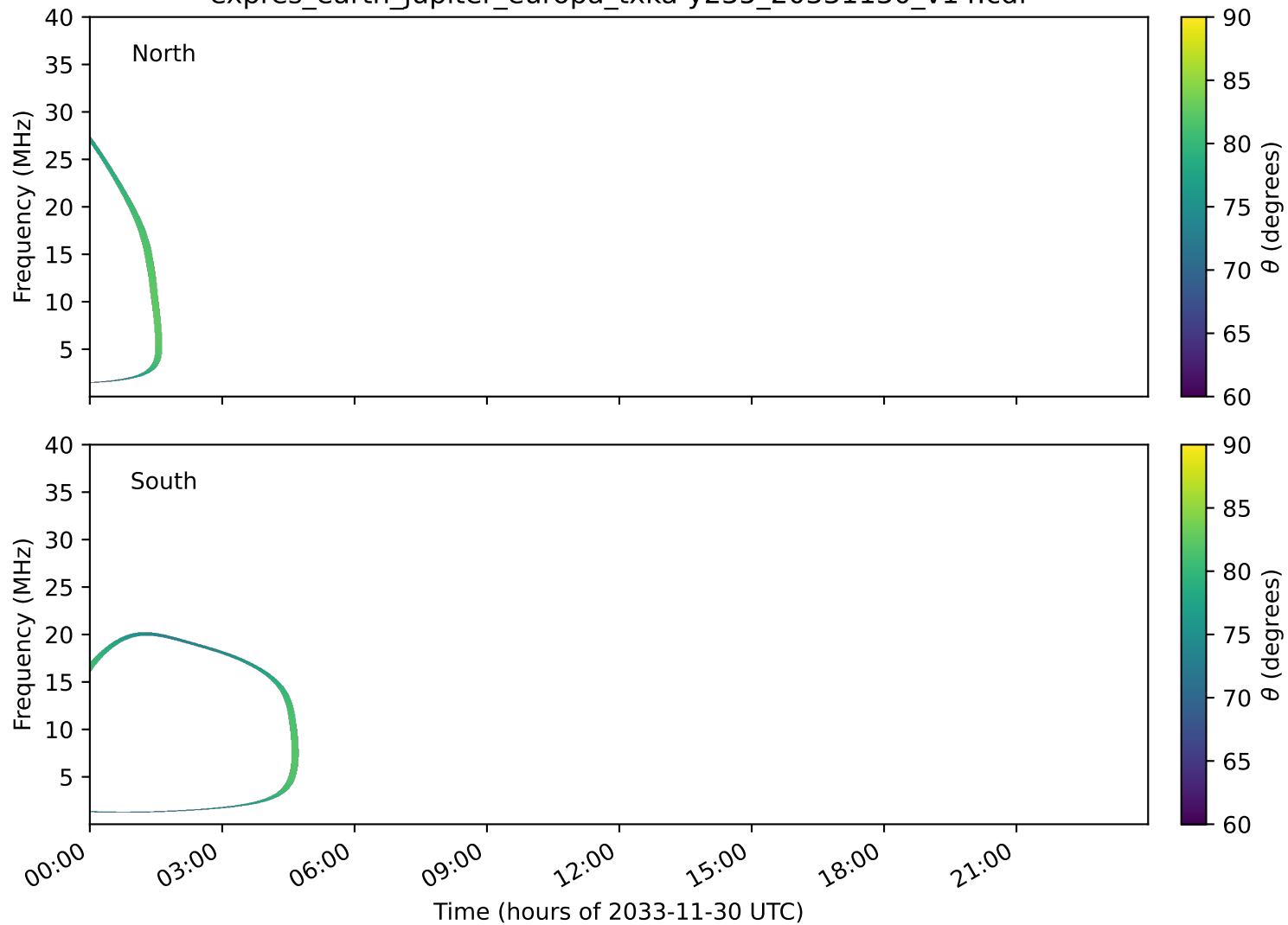
expres_earth_jupiter_europa_txka-y235_20331130_v14.cdf
