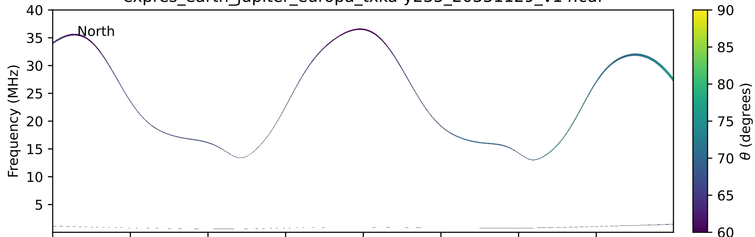
expres_earth_jupiter_europa_txka-y235_20331129_v14.cdf
