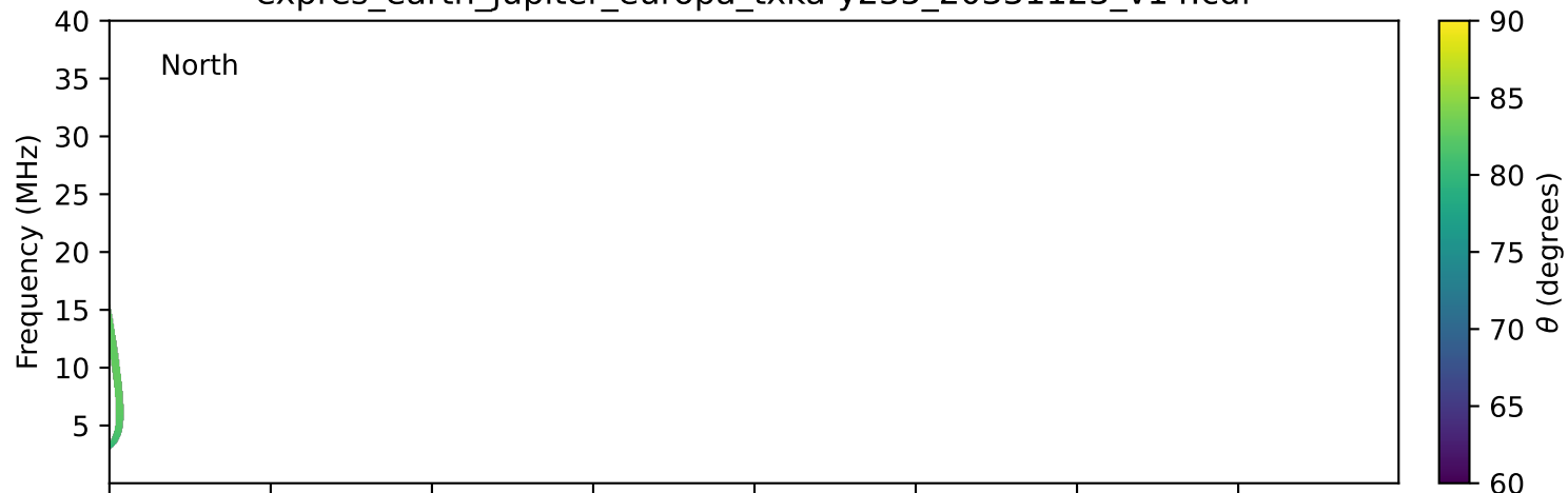
expres_earth_jupiter_europa_txka-y235_20331123_v14.cdf
