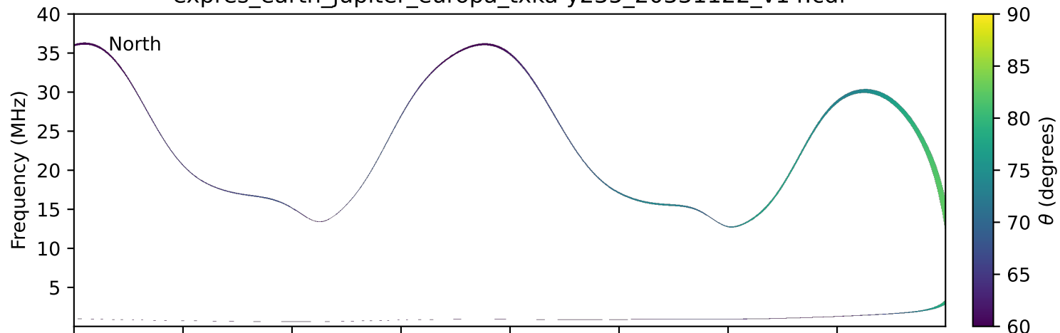
expres_earth_jupiter_europa_txka-y235_20331122_v14.cdf
