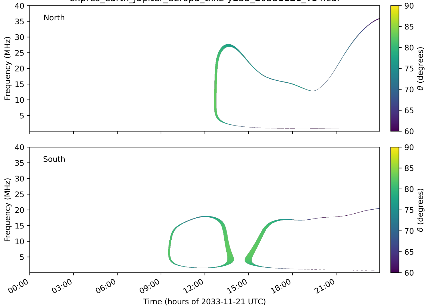
expres_earth_jupiter_europa_txka-y235_20331121_v14.cdf
