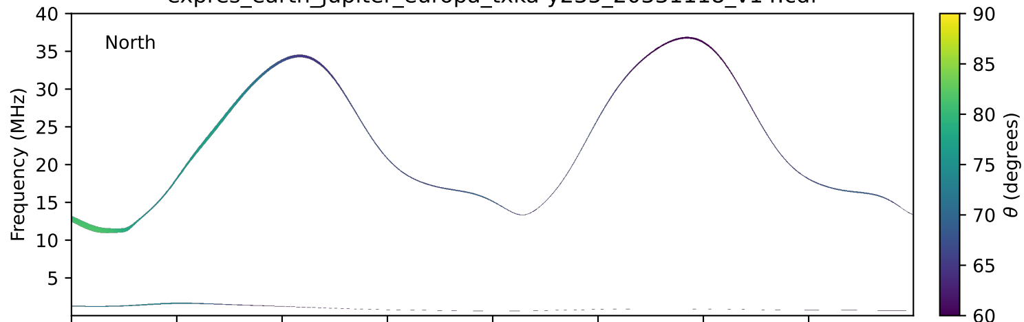
expres_earth_jupiter_europa_txka-y235_20331118_v14.cdf
