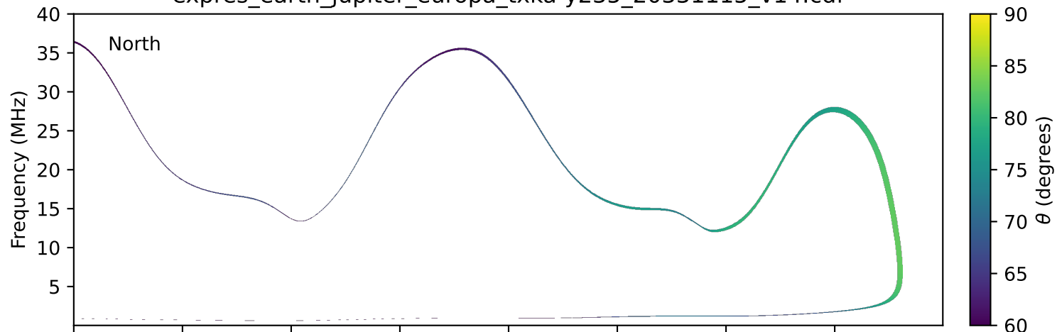
expres_earth_jupiter_europa_txka-y235_20331115_v14.cdf
