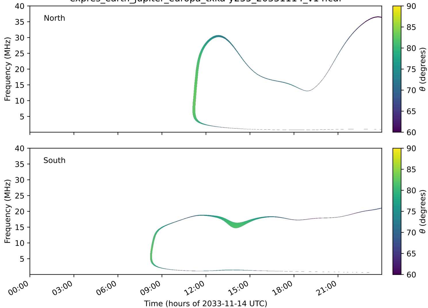
expres_earth_jupiter_europa_txka-y235_20331114_v14.cdf
