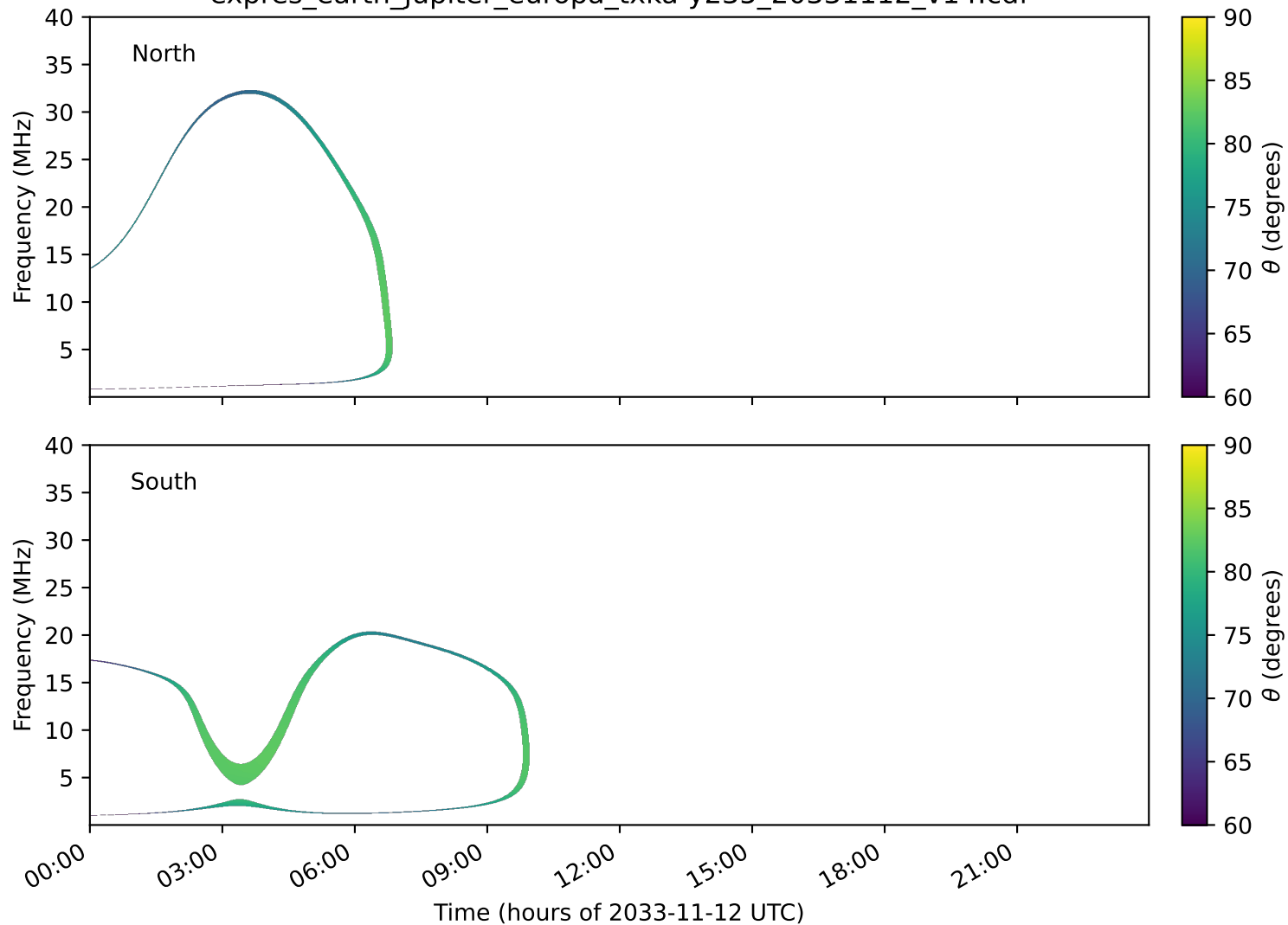
expres_earth_jupiter_europa_txka-y235_20331112_v14.cdf
