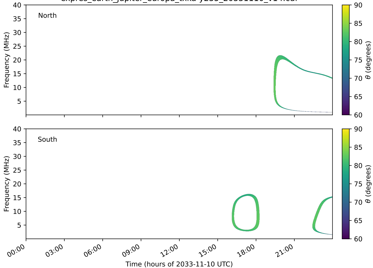
expres_earth_jupiter_europa_txka-y235_20331110_v14.cdf
