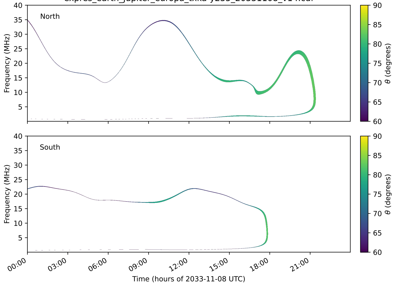
expres_earth_jupiter_europa_txka-y235_20331108_v14.cdf
