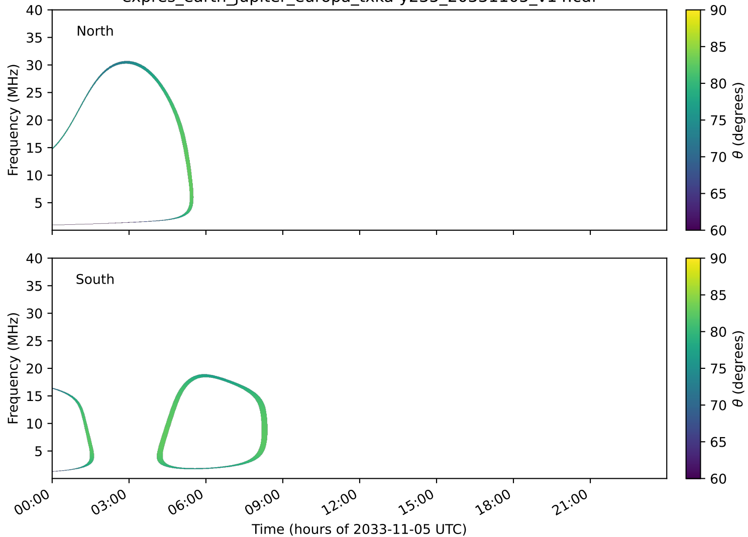
expres_earth_jupiter_europa_txka-y235_20331105_v14.cdf
