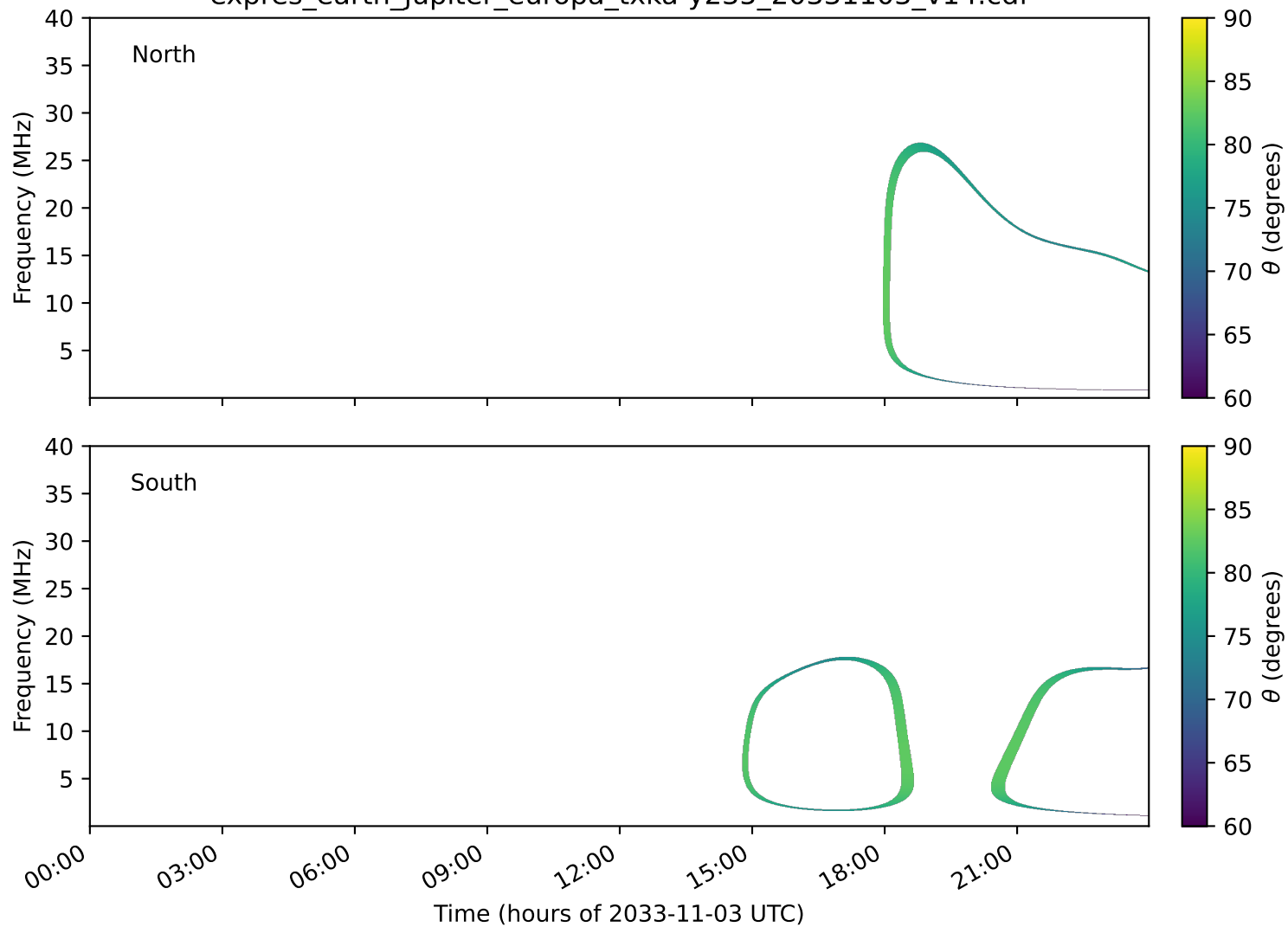
expres_earth_jupiter_europa_txka-y235_20331103_v14.cdf
