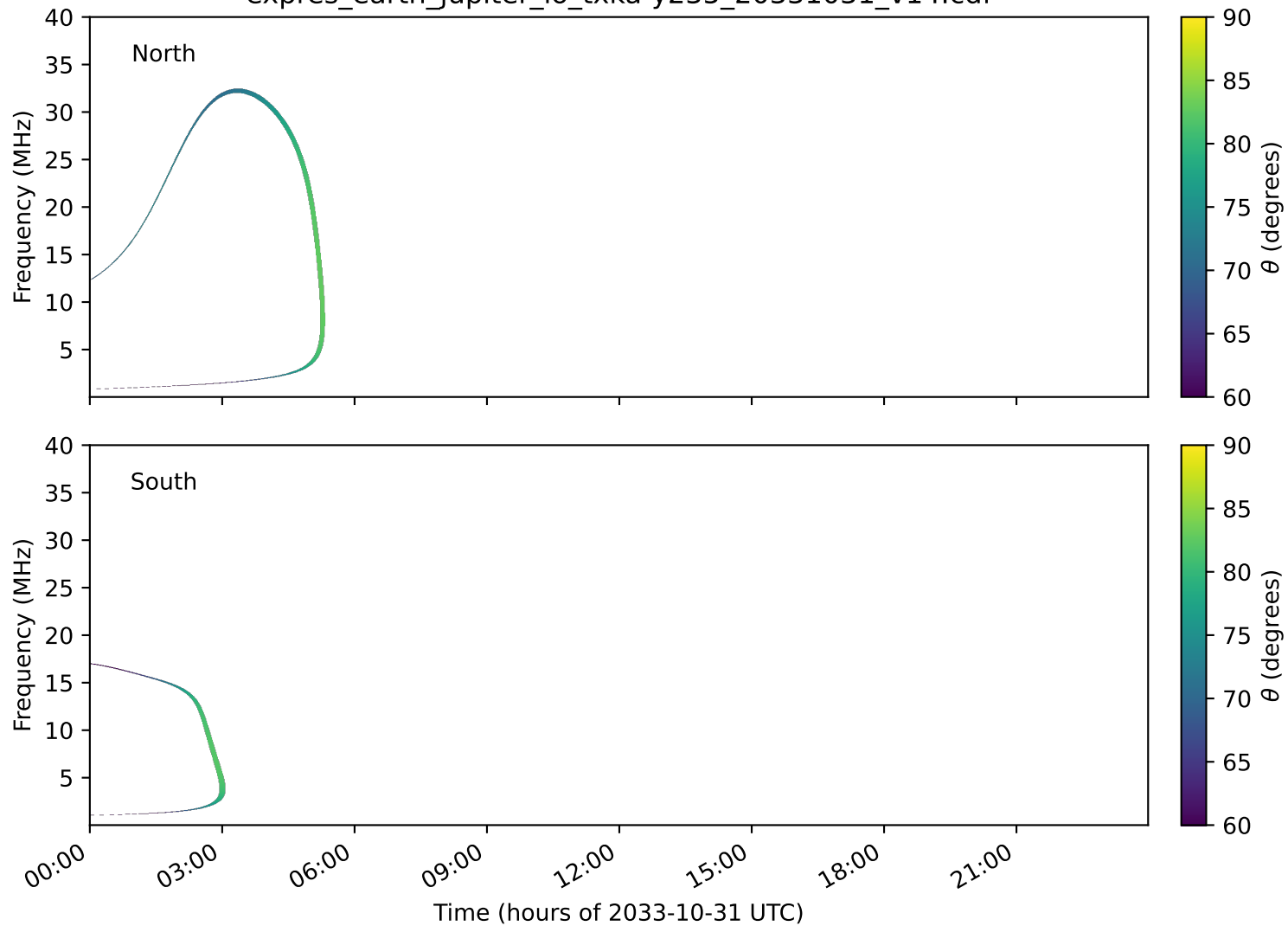
expres_earth_jupiter_io_txka-y235_20331031_v14.cdf
