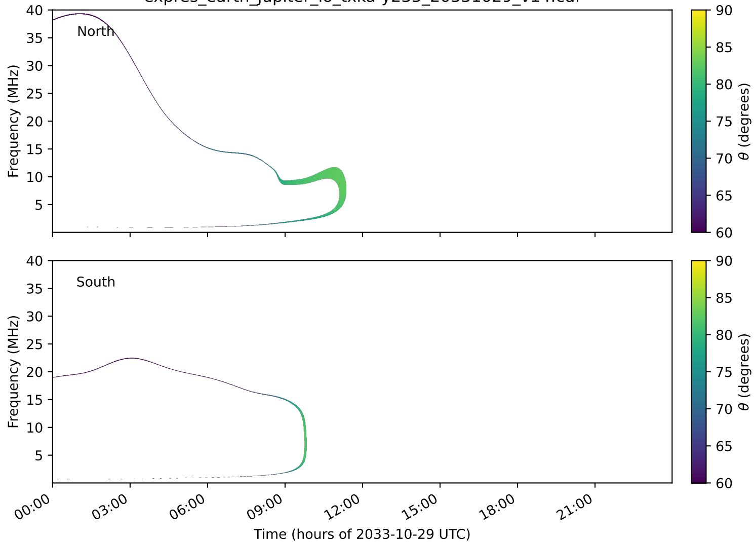
expres_earth_jupiter_io_txka-y235_20331029_v14.cdf
