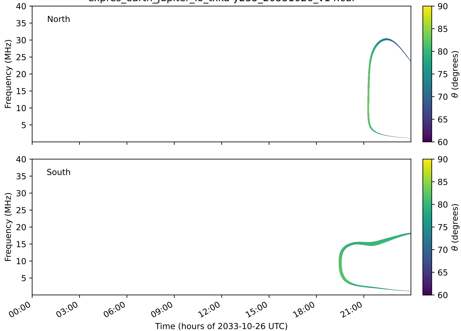
expres_earth_jupiter_io_txka-y235_20331026_v14.cdf
