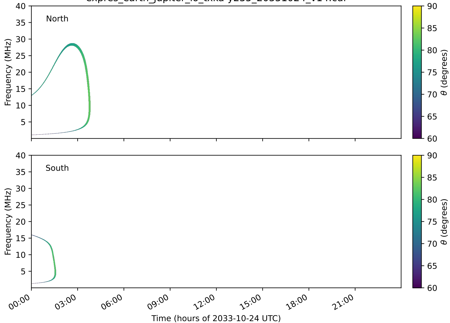
expres_earth_jupiter_io_txka-y235_20331024_v14.cdf
